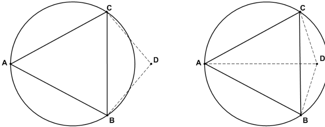
Figure 9 – Circumcircle criteria used for Delaunay triangulations
